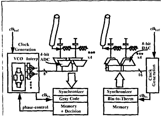
Figure 4.1.1: System architecture.
