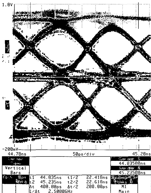
Figure 4.3.6: Signaling rate on four links.
