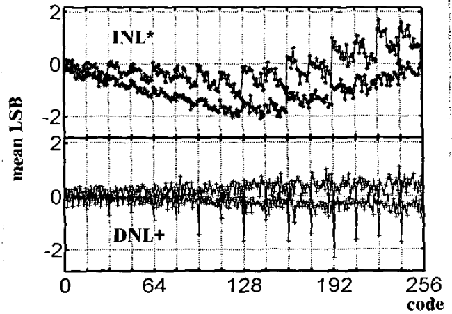
Figure 4.1.4: INL/DNL envelopes for DACs, LSB=2.2mV.
