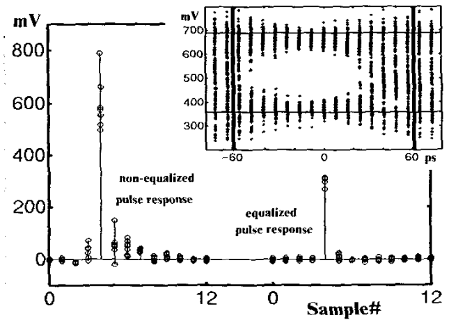
Figure 4.1.6: Transceiver pulse response and equalized eye.
