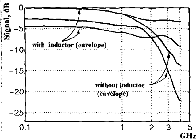
Figure 4.1.5: Transceiver frequency response w/ & w/o inductors.
