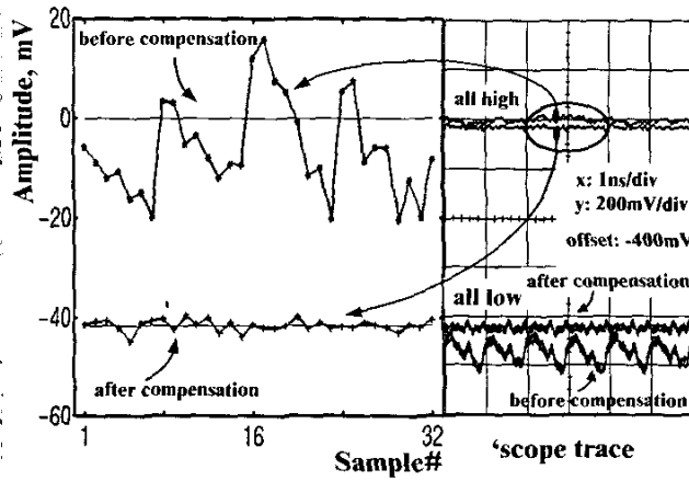
Figure 4.1.3: Transmitter DC coupling.
