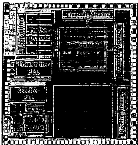
Figure 4.1.7: Chip micrograph.
