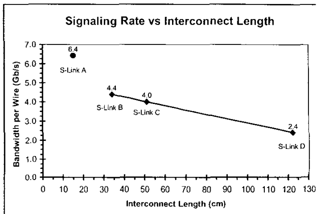
Figure 4.3.6: Signaling rate on four links.
